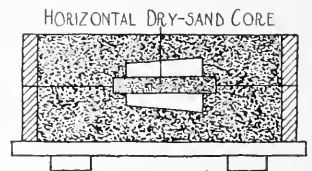
FIG. 535. HORIZONTAL DRY-SAND CORE.
